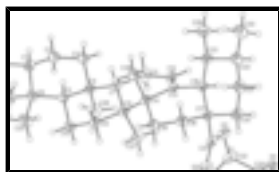
Fig. 1. The molecular structure of (I), showing displacement ellipsoids at the 70% probability level.
