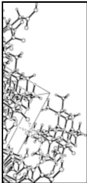
Fig. 2. A packing diagram of (I).
